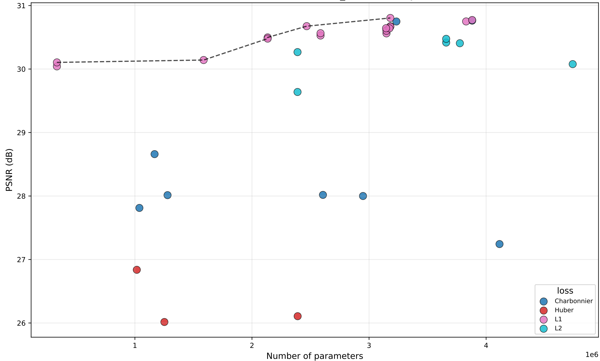
PSNR vs #Params — DHTCUN_baseline — by loss
